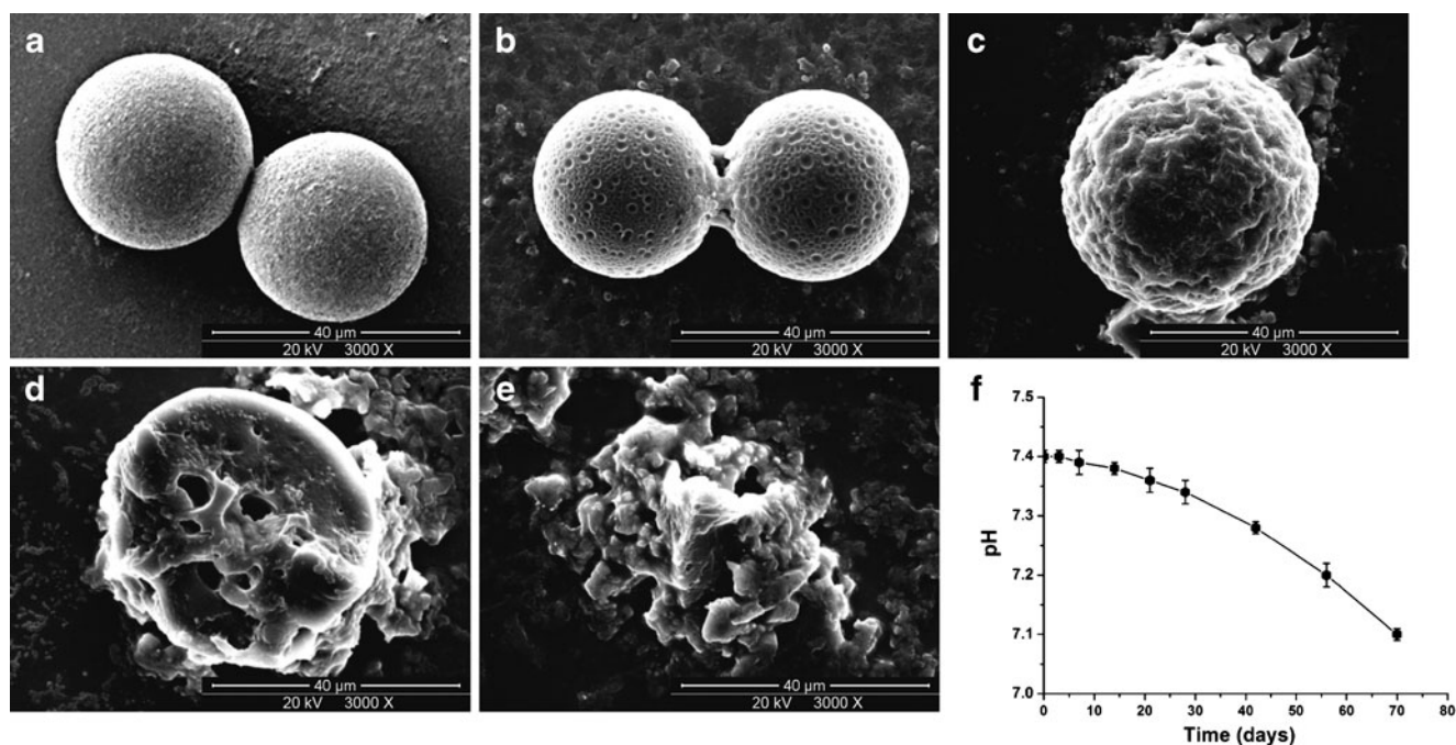
Fig. 3. 25OHD-loaded microspheres produced at 0.4% PVA ( w/v ), 4% PLA ( w/v ), and 1,000 rpm (formula 3) were incubated in PBS (pH 7.4) at 37°C; images of degradation were obtained using scanning electron microscopy. a–e Microspheres after incubation for 0, 7, 28, 56, and 70 days, respectively. f Degradation medium pH
